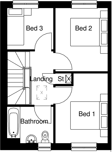
First Floor. 1 : 100
