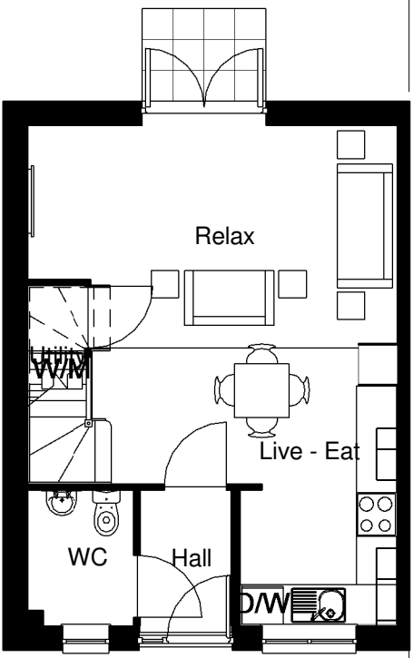
Ground Floor. 1 : 100
